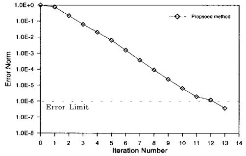
Fig. 12 Error norm versus iteration number of the 10th eigenpair in case of shift = 1.00001\lambda_2
