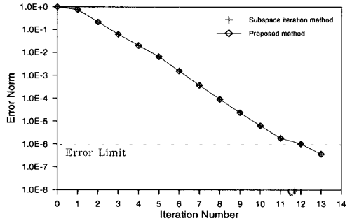
Fig. 10 Error norm versus iteration number of the 10th eigenpair in case of shift = 1.01\lambda_2
