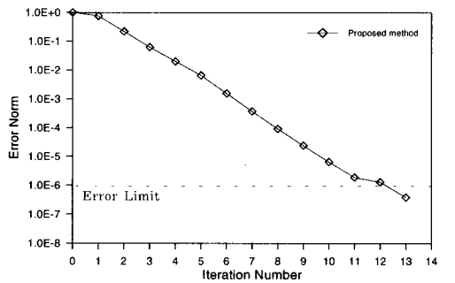
Fig. 14 Error norm versus iteration number of the 10th eigenpair in case of shift = \lambda_2
