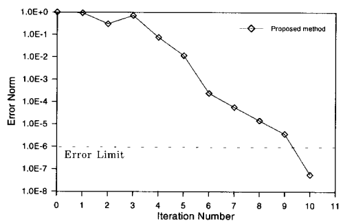
Fig. 7 Error norm versus iteration number of the 10th eigenpair in case of shift = \lambda_4
