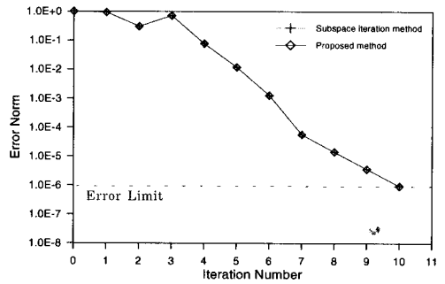
Fig. 3 Error norm versus iteration number of the 10th eigenpair in case of shift = 1.01\lambda_4
