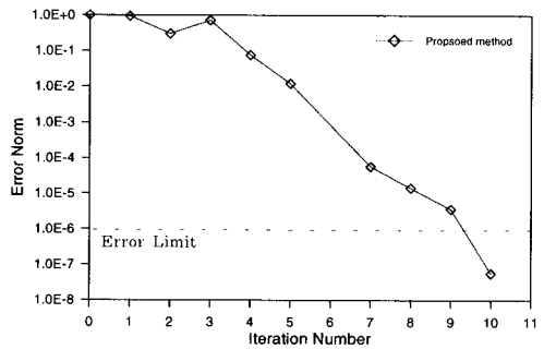
Fig. 5 Error norm versus iteration number of the 10th eigenpair in case of shift = 1.00001\lambda_4
