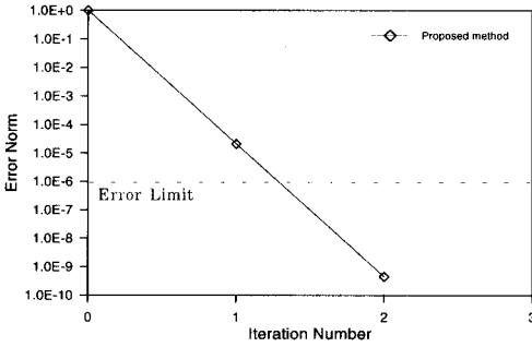
Fig. 11 Error norm versus iteration number of the 2nd eigenpair in case of shift = 1.00001\lambda_2
