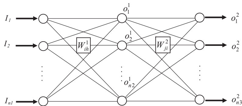
Fig. 1. Structure of multi-layer perceptron with one hidden layer.
