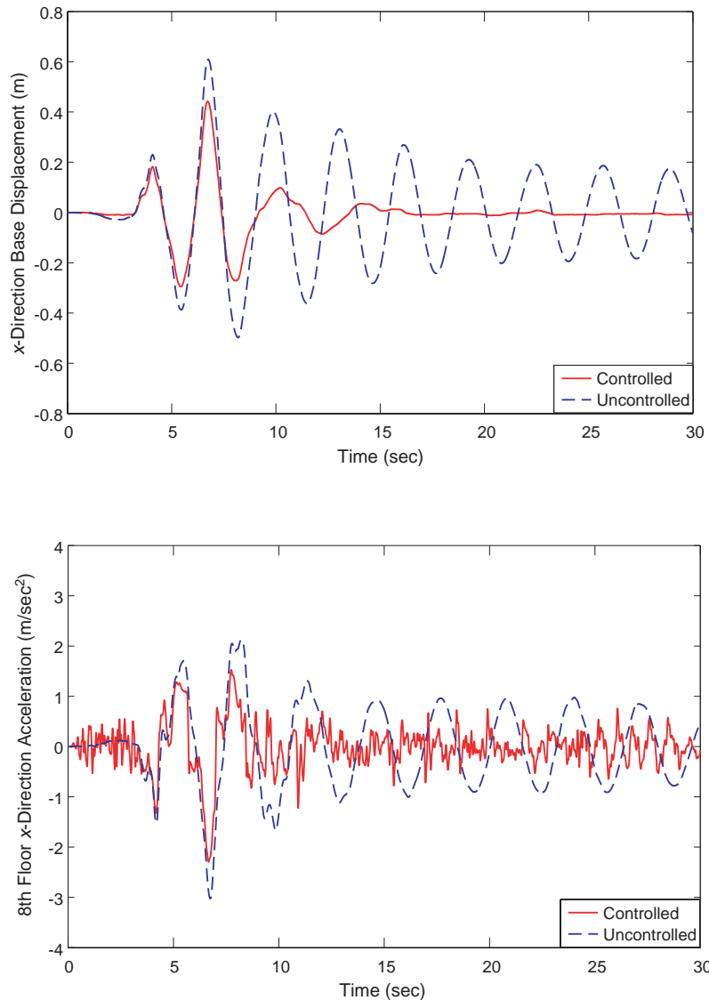
Fig. 5. Performance of the neuro-controller under Sylmar earthquake (FP-X, FN-Y)
