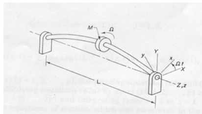
Figure 1. Whirling Beam
